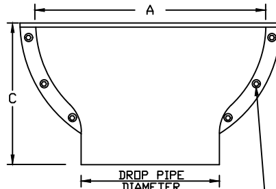
DROP BOWL FRONT VIEW
