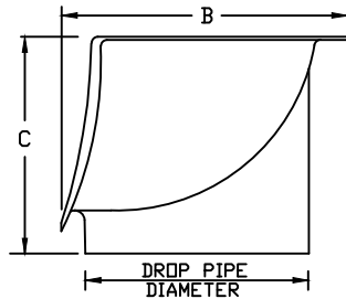
DROP BOWL SIDE VIEW
